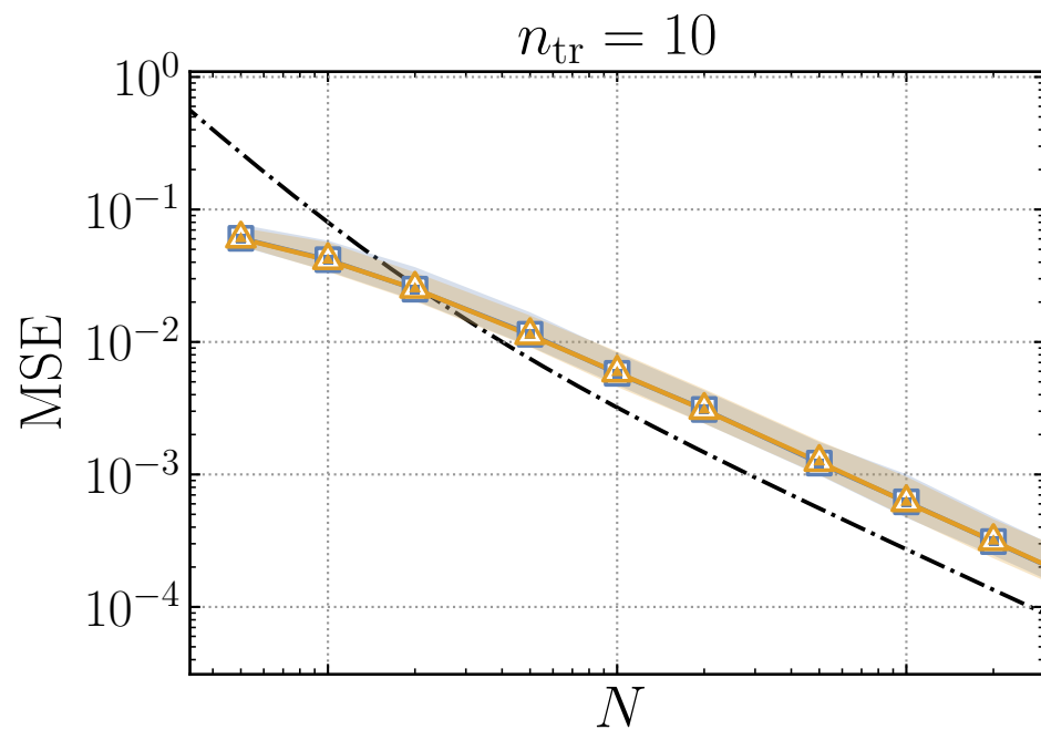
MSE vs N : multinomial vs. Gaussian approx. ( d = 2 , 100 instances)
